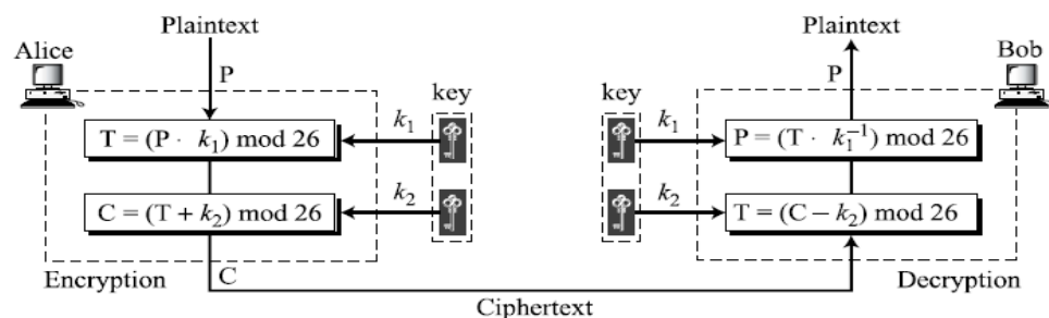
Figure 3.11 Affine cipher
